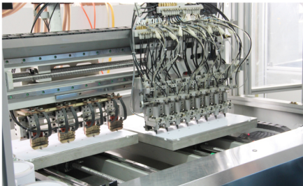
Contactless IC Encapsulation
