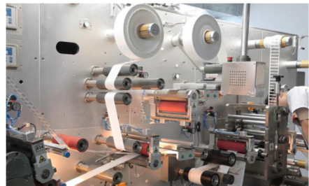
RFID Tag Automatical Compound Machine
